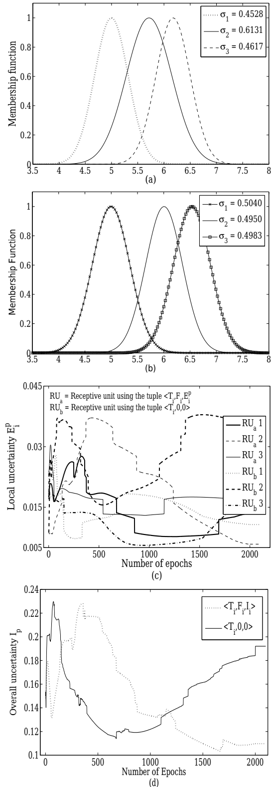
Fig. 6: (a) Final distribution using the tuple \langle T, 0, 0 \rangle , (b) Final distribution using the tuple \langle T, F, I_k \rangle , (c) local uncertainty E_j^k performance and (d) Overall uncertainty I_k produced by the overlapping among the RUs throughout the training process
