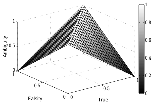
Fig. 4: Ambiguity ( I_{ik}^p )
