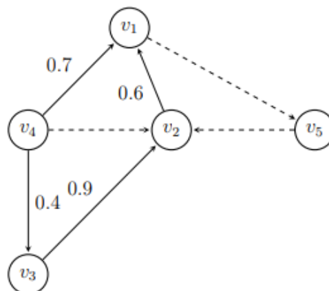
Figure 1. Neutrosophic Cognitive Maps example.
