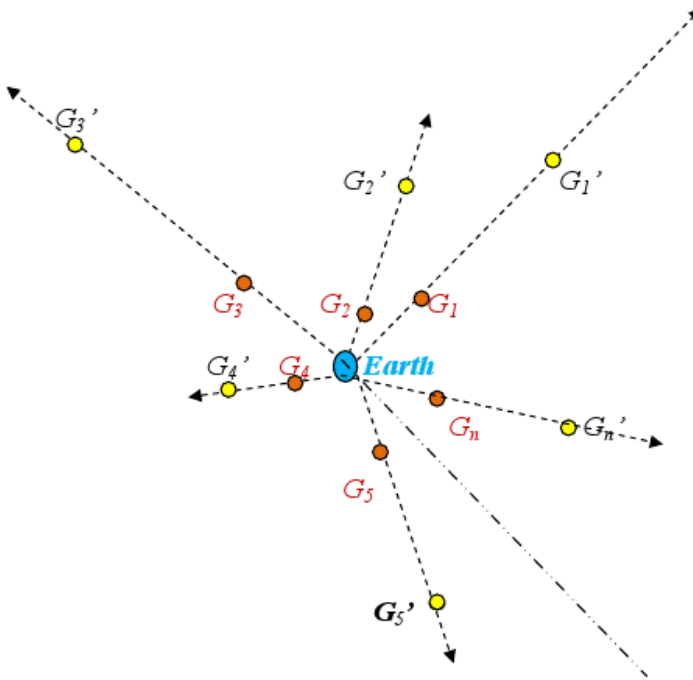
Fig. 31. Diagram of Allegedly Expansion Universe
