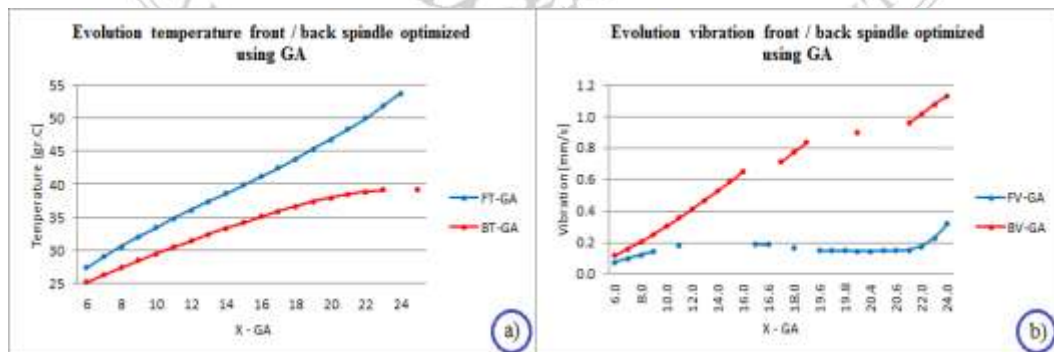
Fig. 4. Evolution of temperatures/vibrations front/back to the general spindle with solution optimization using genetic algorithms.
