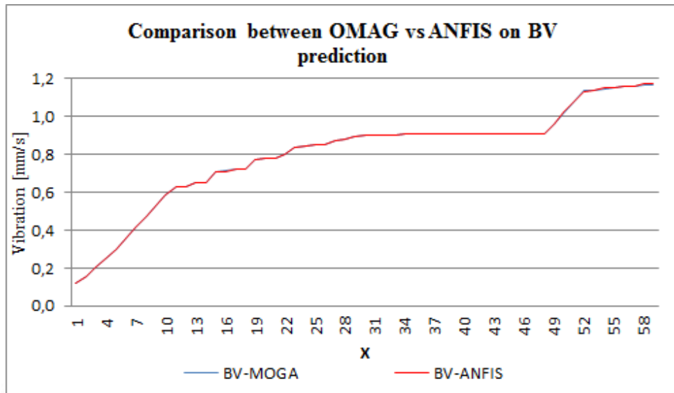
Fig. 12. Comparison between OMAG and ANFIS on BV prediction.
