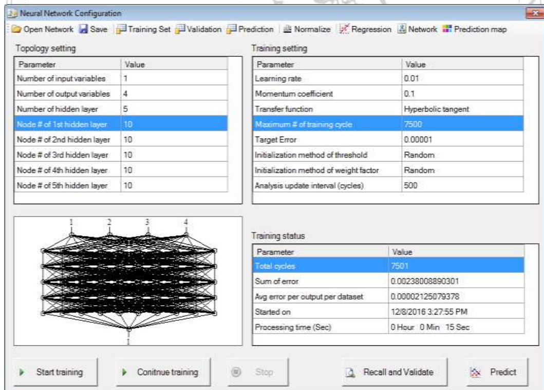
Fig. 6. Configuring artificial neural network using Visual Gene Developer 1.7 software.
