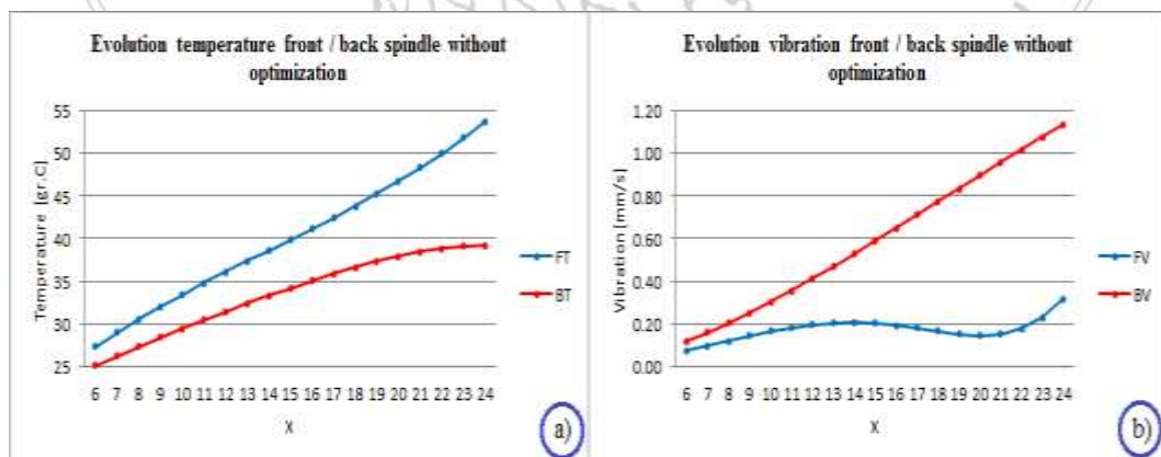
Fig. 3 Evolution temperature/vibration front/back spindle generally without optimization solutions.
