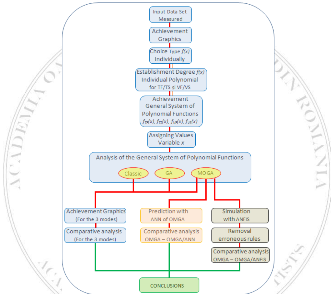
Fig. 1. Scheme of the algorithm.
