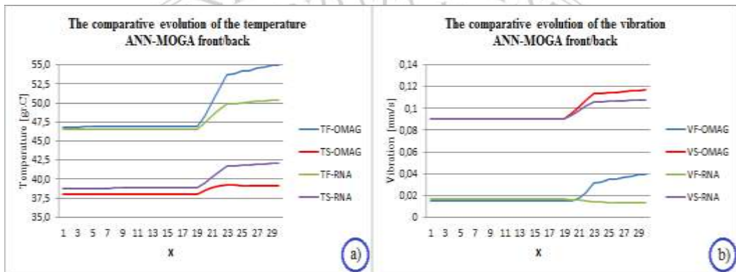
Fig. 8. MOGA-ANN Comparative evolution MOGA-ANN of front/back temperatures /vibrations. front/back
