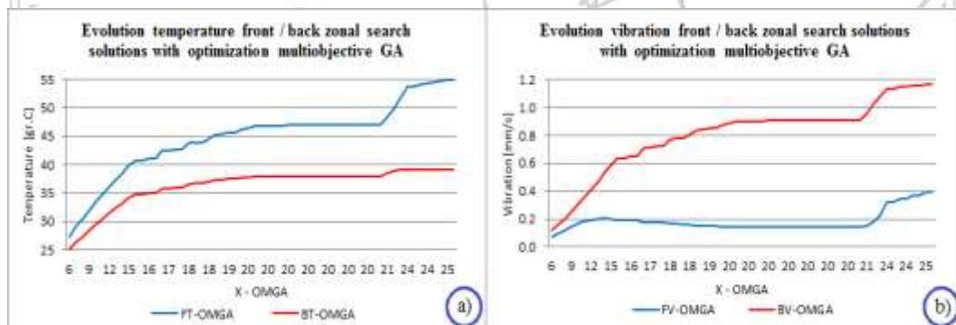
Fig. 5. Evolution temperatures/vibrations front/back to the general spindle using multi-objective optimization with genetic algorithms.
