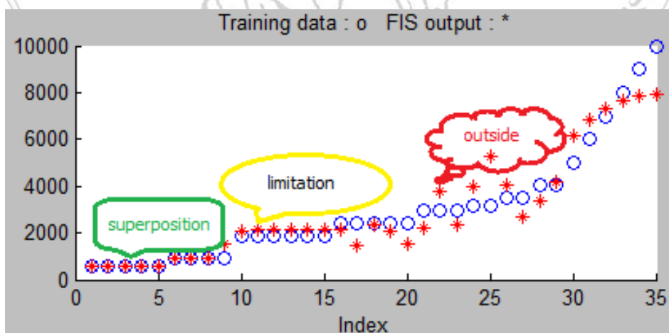
Fig. 10. Possible types of errors that occur during training.
