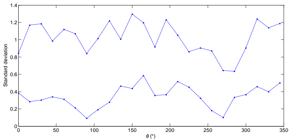
Figure 4. The neutrosophic standard deviations of JRC-NNs in different orientations \theta .
