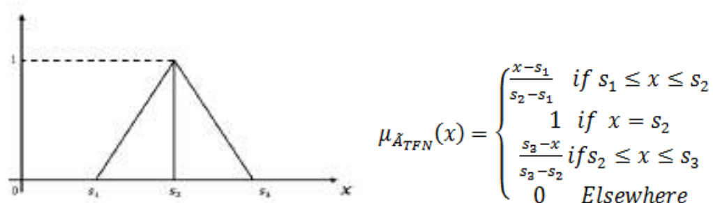
Figure 2.5.3.1: Graphical Representation of Linear Triangular Fuzzy Number
