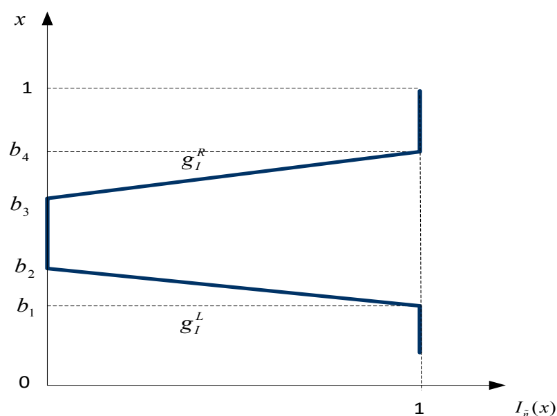
Figure 4. Indeterminate membership function of trapezoidal fuzzy neutrosophic set with centroid
