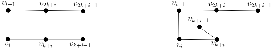
Figure 2: Two possible drawings of E_i
