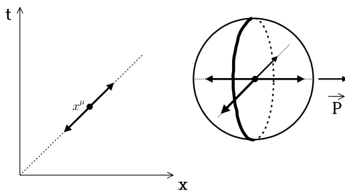
Fig. 1: Contributions of spinors at x^\mu .
