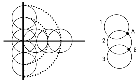
Fig. 2: Formation of simultaneous wavefronts.
