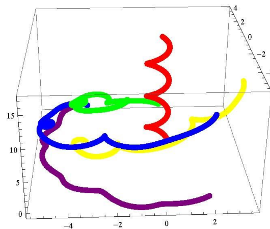
Figure 5. \gamma and its Bishop adjoint curves.
