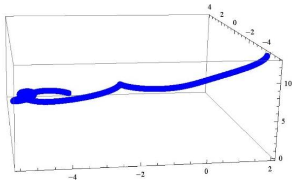
Figure 4. \mathbf{t}_\gamma \zeta_1^\gamma \zeta_2^\gamma -Bishop adjoint curve.
