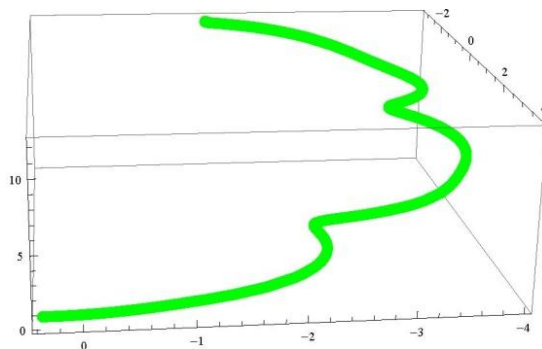
Figure 1. \mathbf{t}_\gamma \zeta_1^\gamma -Bishop adjoint curve.
