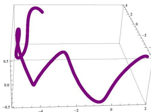
Figure 3. \zeta_1^\gamma \zeta_2^\gamma -Bishop adjoint curve.
