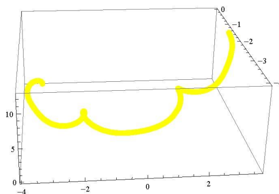
Figure 2. \mathbf{t}_\gamma \zeta_2^\gamma -Bishop adjoint curve.
