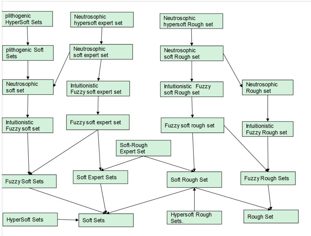
FIGURE 7. Some Soft Sets and Rough Sets Hierarchy. The Set class at the origin of an arrow contains the set class at the destination of the arrow.
