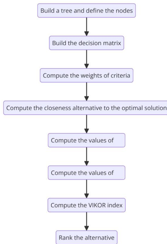
Figure 1. TreeSoft Set with the VIKOR method
